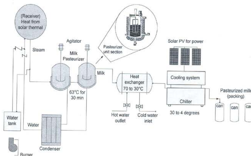
Proposed plan for solar assisted milk pasteurizer
