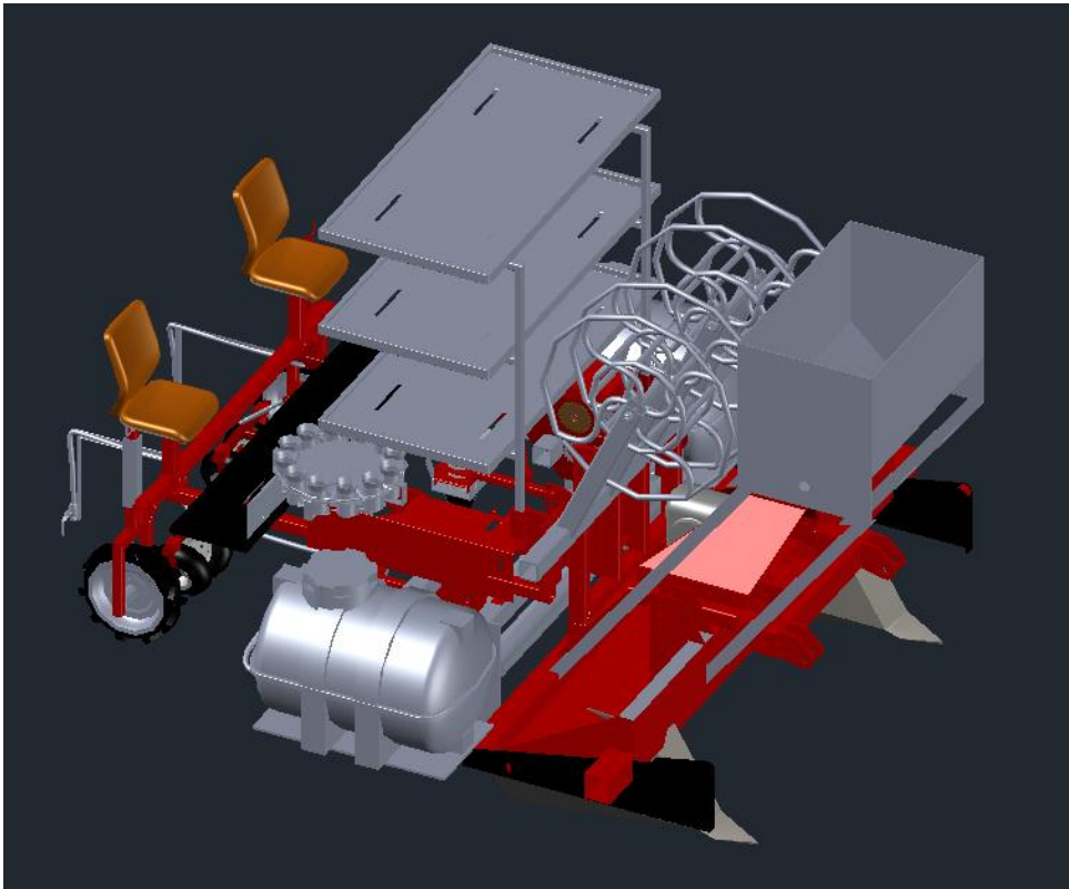
Picture 1. Tractor mounted vegetable nursery transplanter
